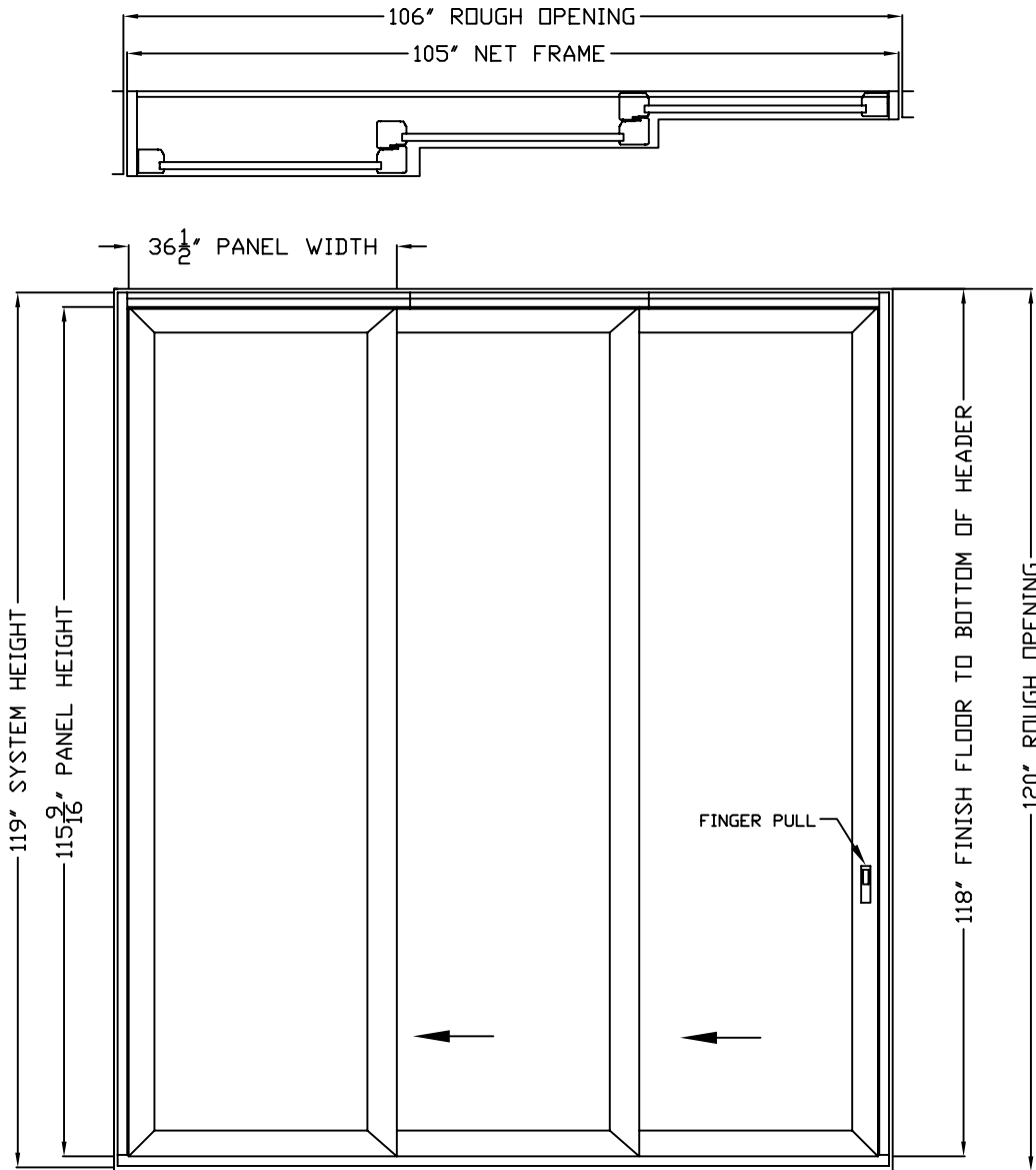
EXTERIOR ELEVATION
